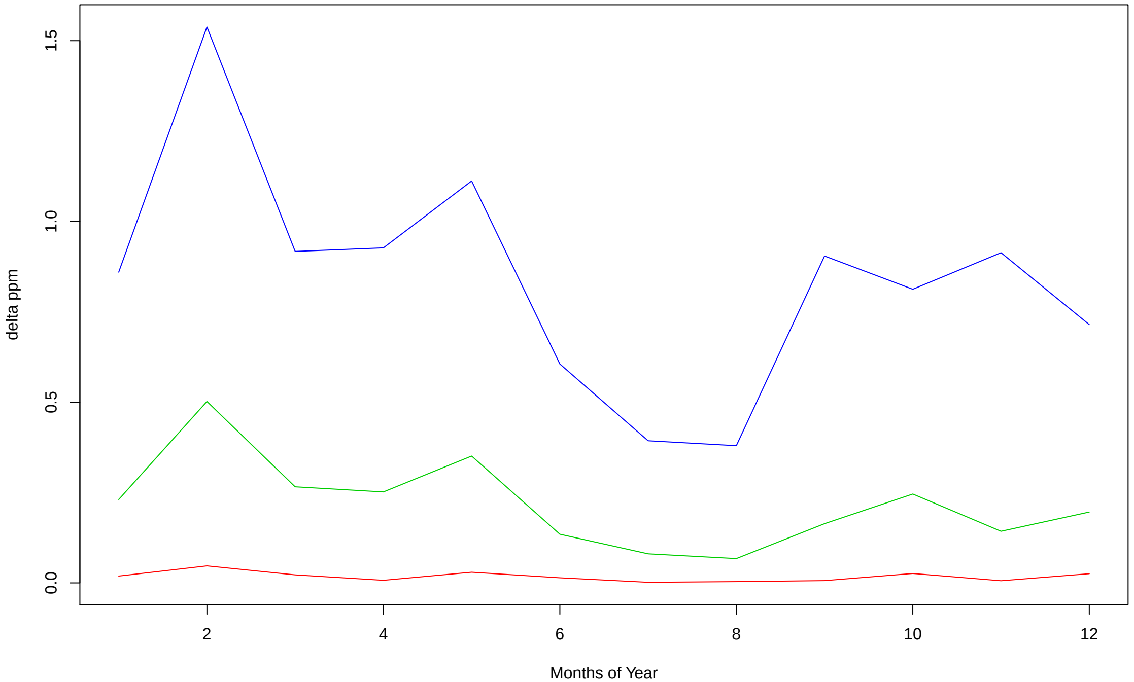
Experiment 1: Delta PPM from SW domain observed at HDP in situ CO2 site
