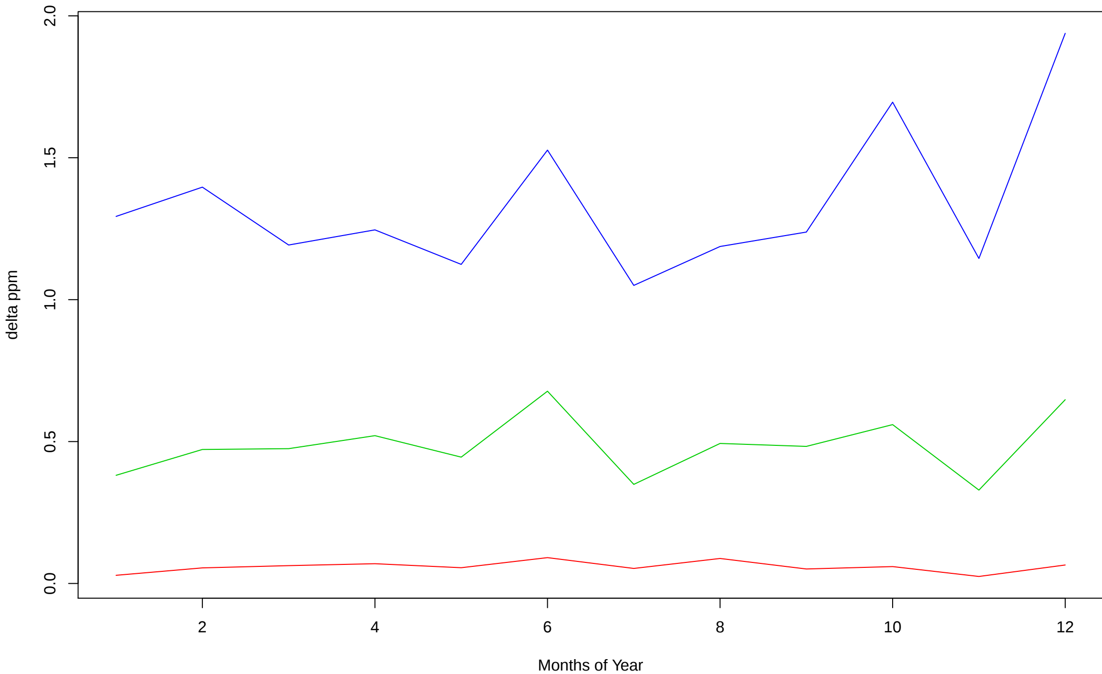
Experiment 0: Delta PPM from NW domain observed at NWR in situ CO2 site
