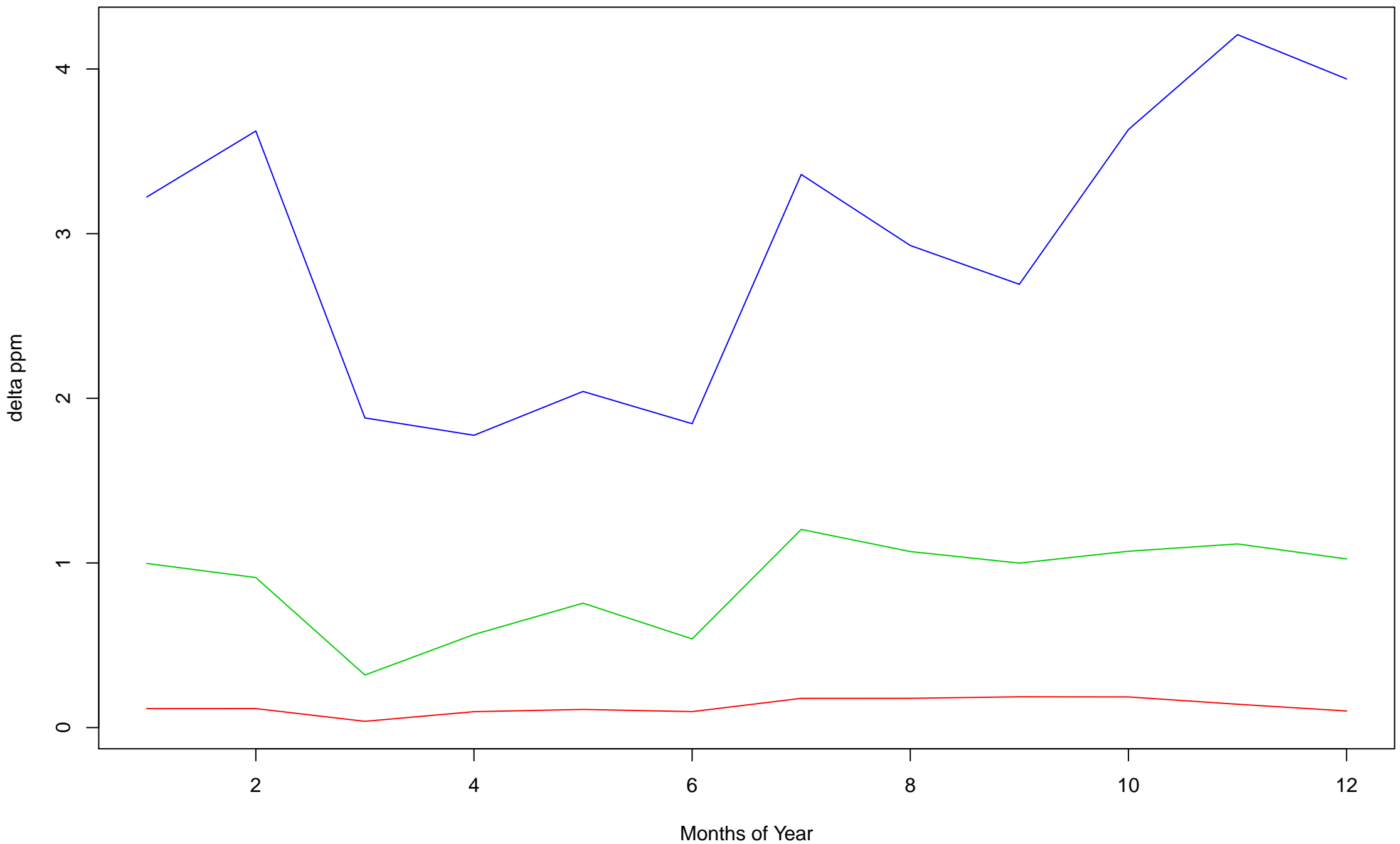
Experiment 0: Delta PPM from NW domain observed at HDP in situ CO2 site
