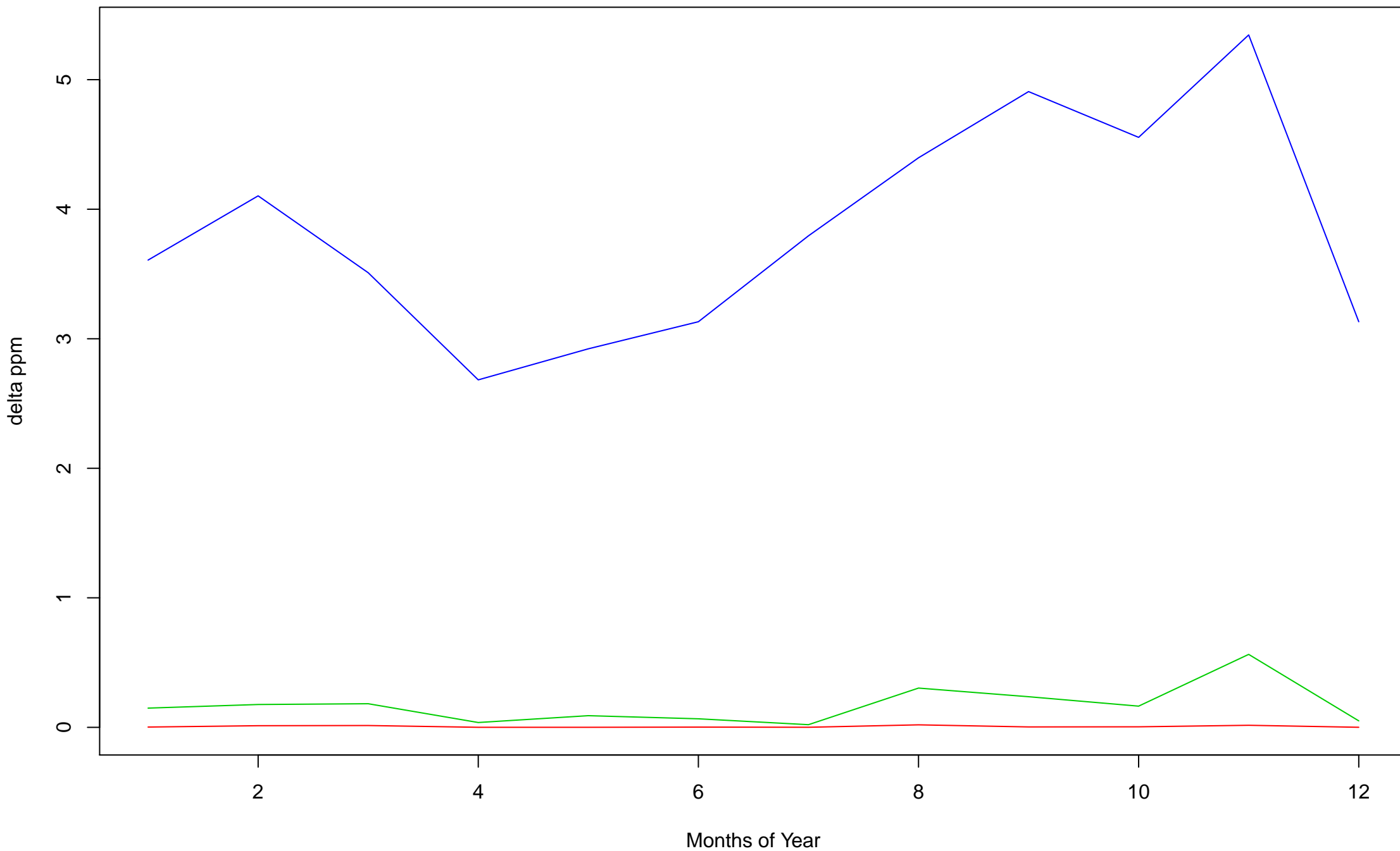
Experiment 0: Delta PPM from ACME domain observed at HDP in situ CO2 site
