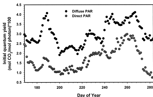
FIG. 8. Seasonal variation of initial quantum yield of a conifer (Scots) pine forest in Finland. Quantum yield is the initial slope of the response between canopy CO 2 exchange and photosynthetic photon flux density. PAR is photosynthetically active radiation.
