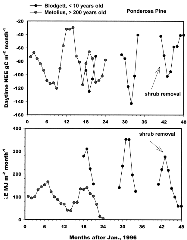
FIG. 13. The impact of stand age on daytime CO_2 exchange (NEE) and latent heat exchange (LE). The data are from a young ( < 10 \text{ yr} ; black circles) and an old ( > 200 \text{ yr} ; gray circles) ponderosa pine forest (see Law et al. 2001, manuscript submitted to Global Change Biol. ; Goldstein et al. 2000).
