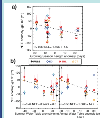
Figure 7. Relationship of climate factor anomalies to regional NEE anomalies for a) growing season length computed by IFUSE model and b) (left) summer minimum water table or (right) 1-yr lagged annual mean water table position observed at the Lost Creek fen.
