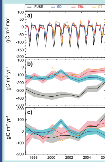
Figure 6. Comparison of regional NEE from the four methods at the a) monthly and b) annual timestep. Also shown is c) annual anomalies in NEE. Error bars were computed by model specific propagation of uncertainties in forcing, parameters, and scaling variables.
