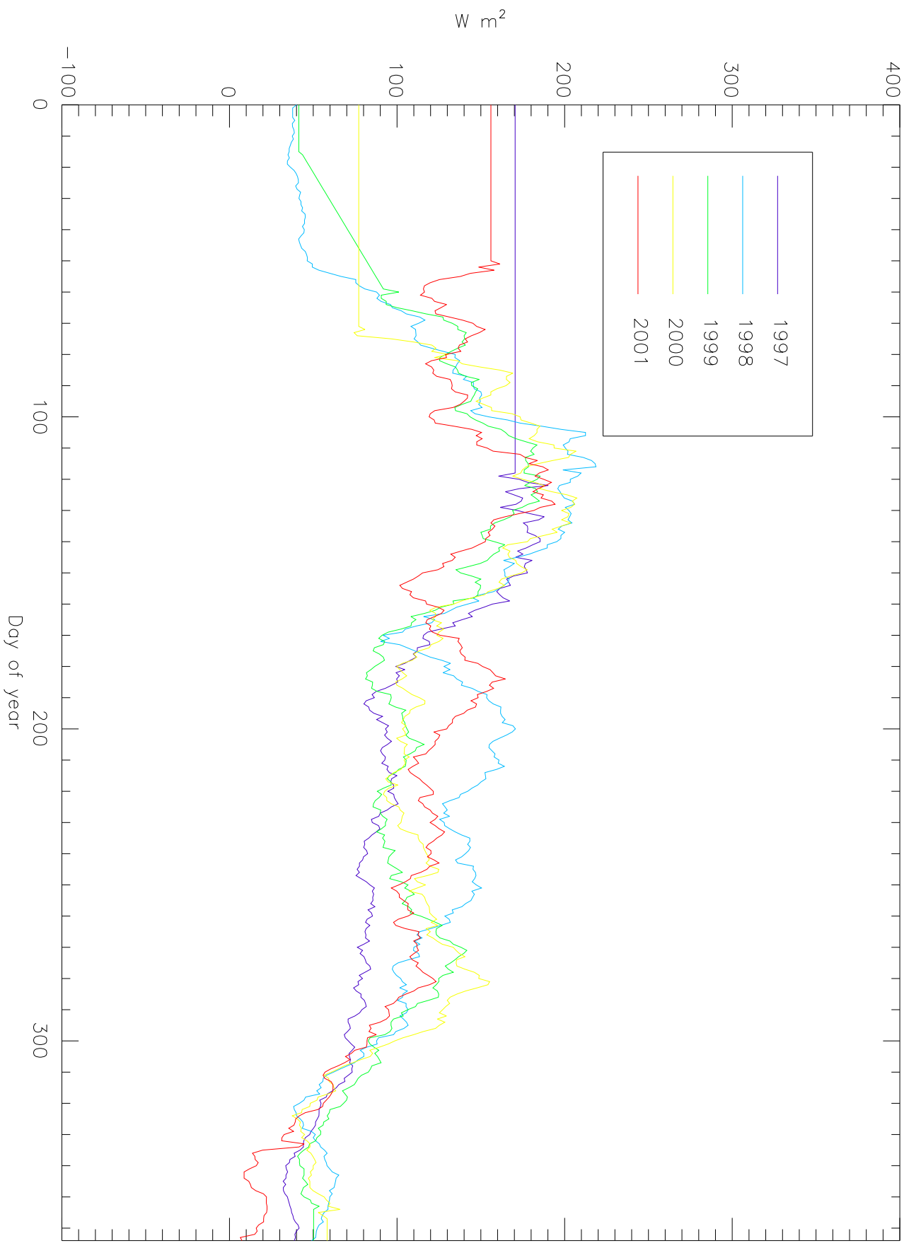
Daytime NEE of sensible heat at WLEF: 1997–2001
