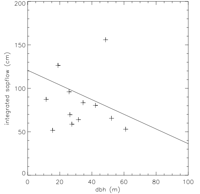
Flow vs DBH SP: YB r^2=0.01 \text{chisq}=14863.51
