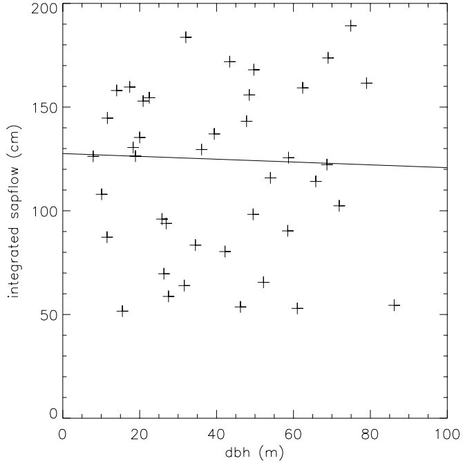
Flow vs DBH SP: SM r^2=0.02 \text{chisq}=27727.96
