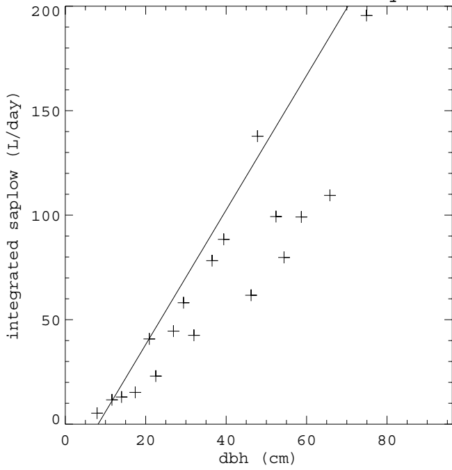
Flow vs DBH SP: SM r^2=0.27 \text{chisq}=216095.75 Flow vs DBH SP: YB r^2=0.70 \text{chisq}=9266.56
