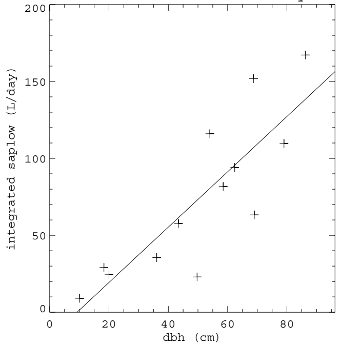
Flow vs DBH SP: SM r^2=0.27 \text{chisq}=216095.75 Flow vs DBH SP: YB r^2=0.70 \text{chisq}=9266.56
