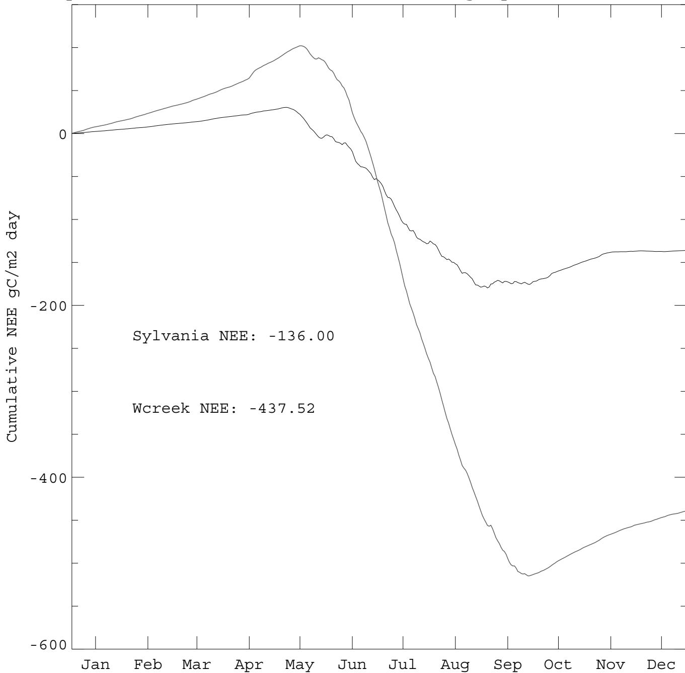
Sylvania (black) vs Willow Creek (gray) cumulative NEE
