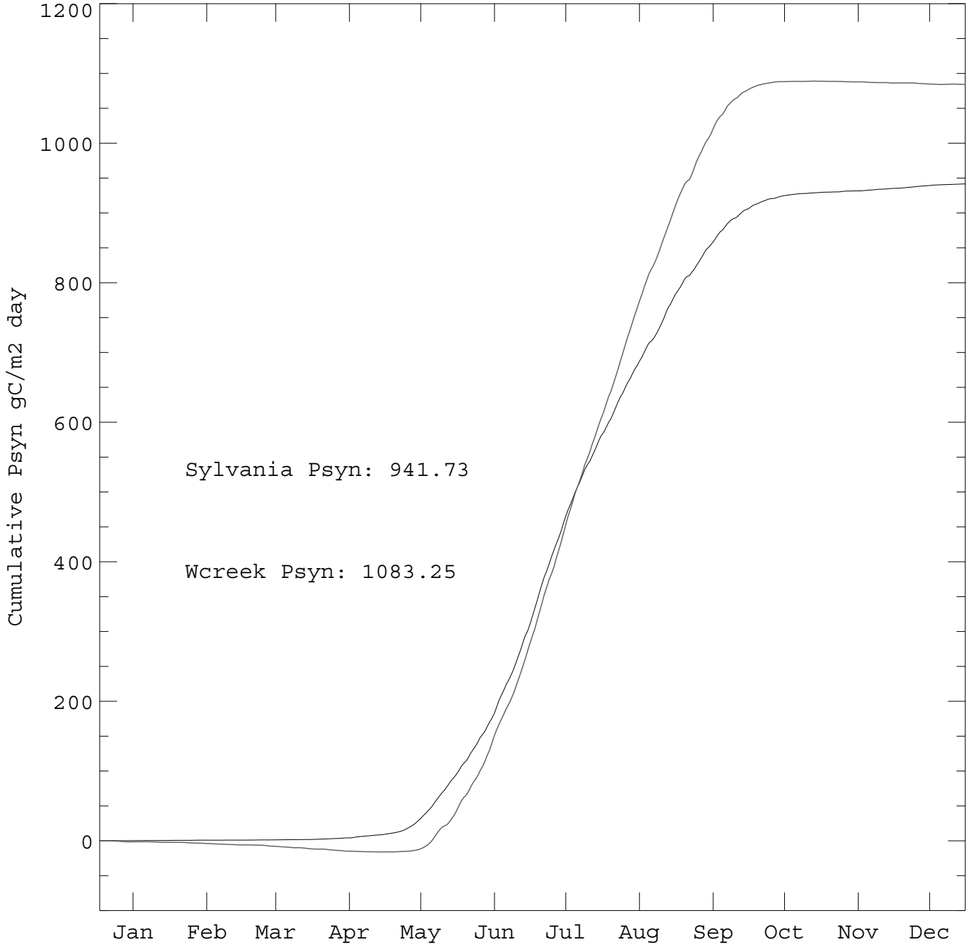
Sylvania (black) vs Willow Creek (gray) cumulative Psyn
