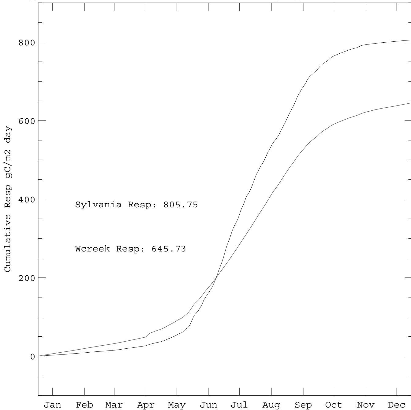
Sylvania (black) vs Willow Creek (gray) cumulative Resp
