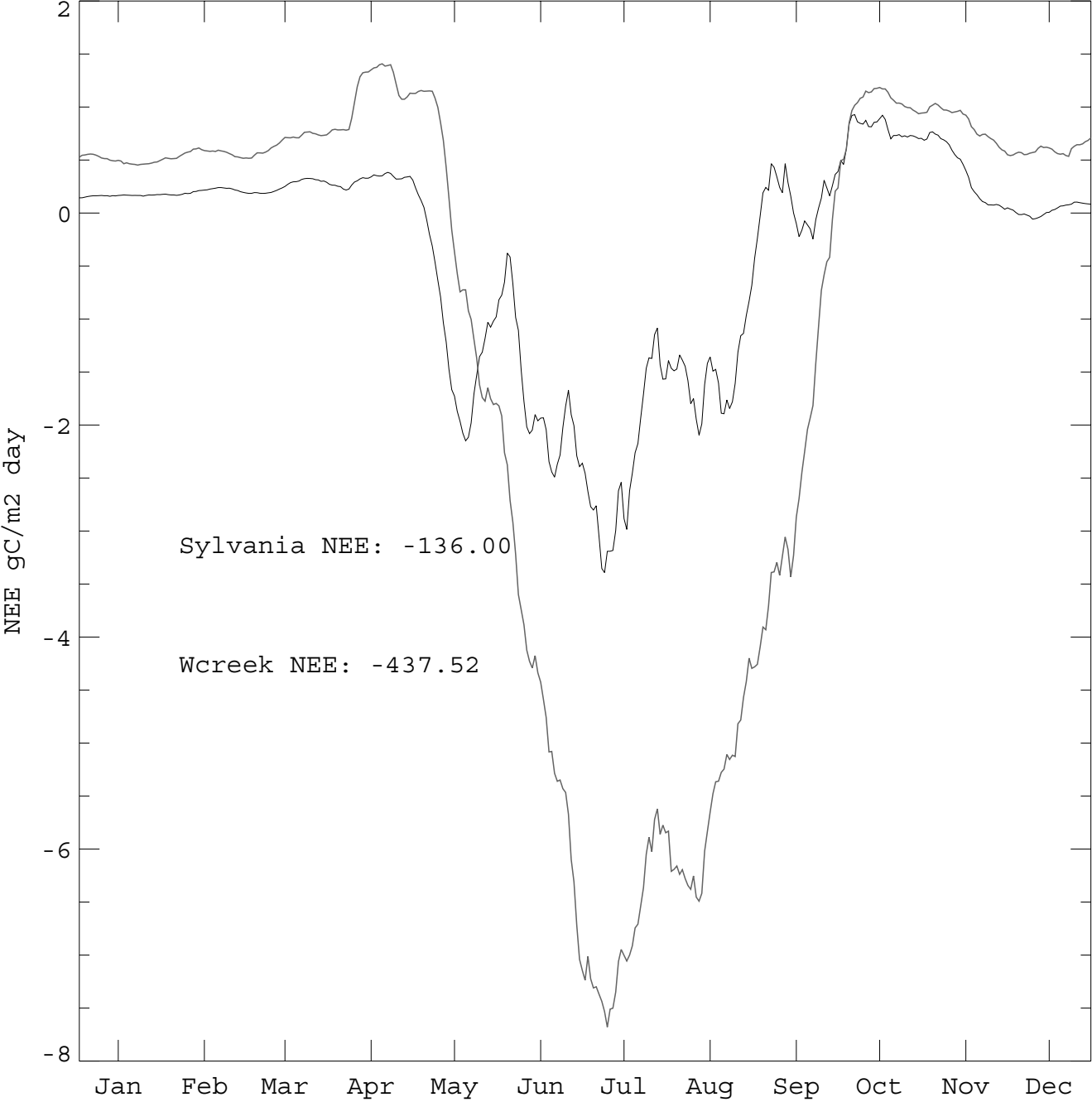
Sylvania (black) vs W.Creek (gray) 2-wk smooth daily NEE
