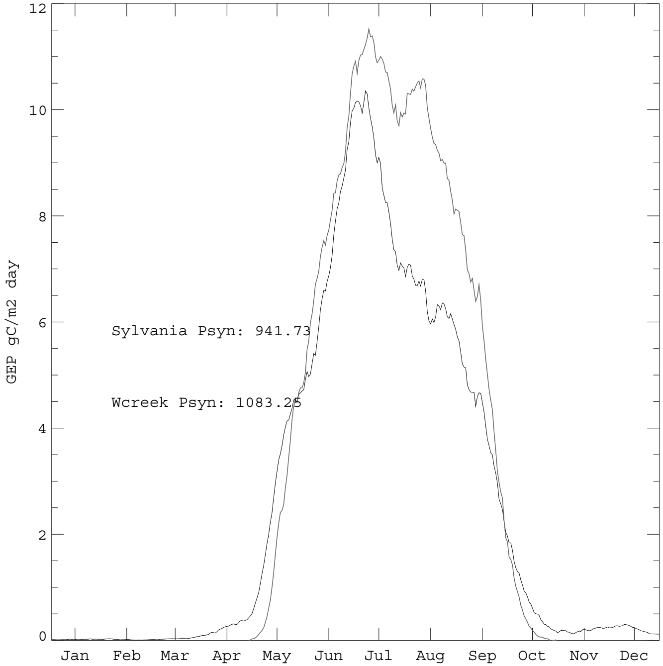
Sylvania (black) vs W.Creek (gray) 2-wk smooth daily Psyn
