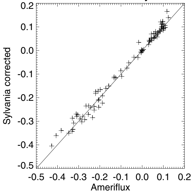
30-min CO2-flux r^2=0.99 y=0.98x+0.0
