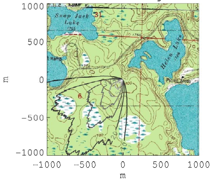
Summer SW Night
