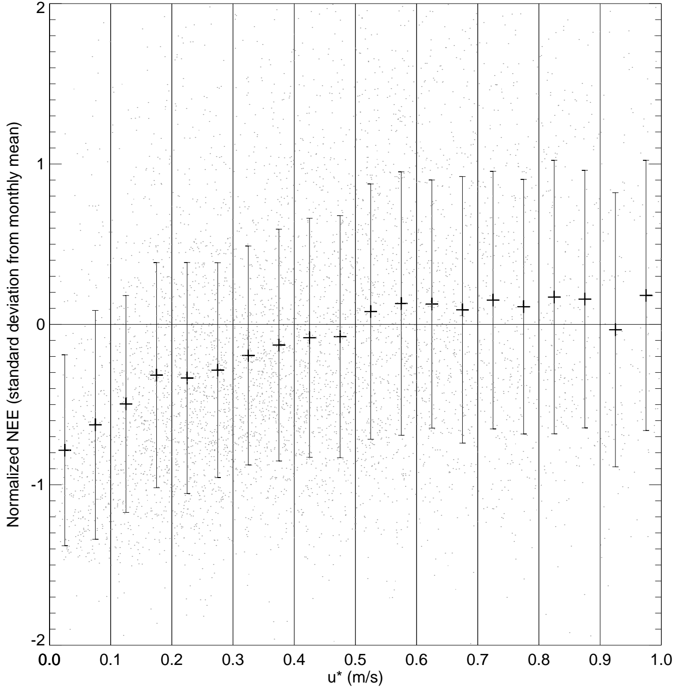
U* vs nighttime NEE Sylvania 2006 Month: 1-12
