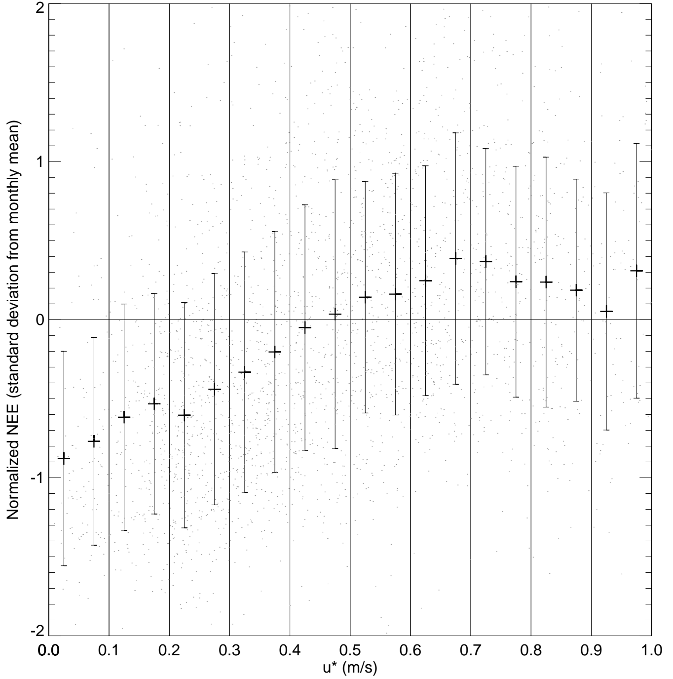
U* vs nighttime NEE Sylvania 2006 Month: 1-12 SOUTH
