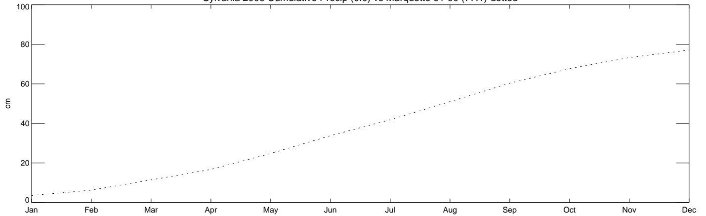
Sylvania 2006 Cumulative Precip (0.0) vs Marquette 61-90 (77.1)-dotted
