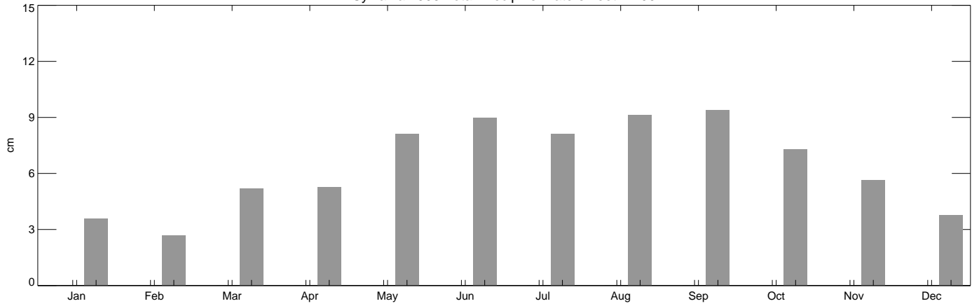
Sylvania 2006 Cumulative Precip (0.0) vs Marquette 61-90 (77.1)-dotted
