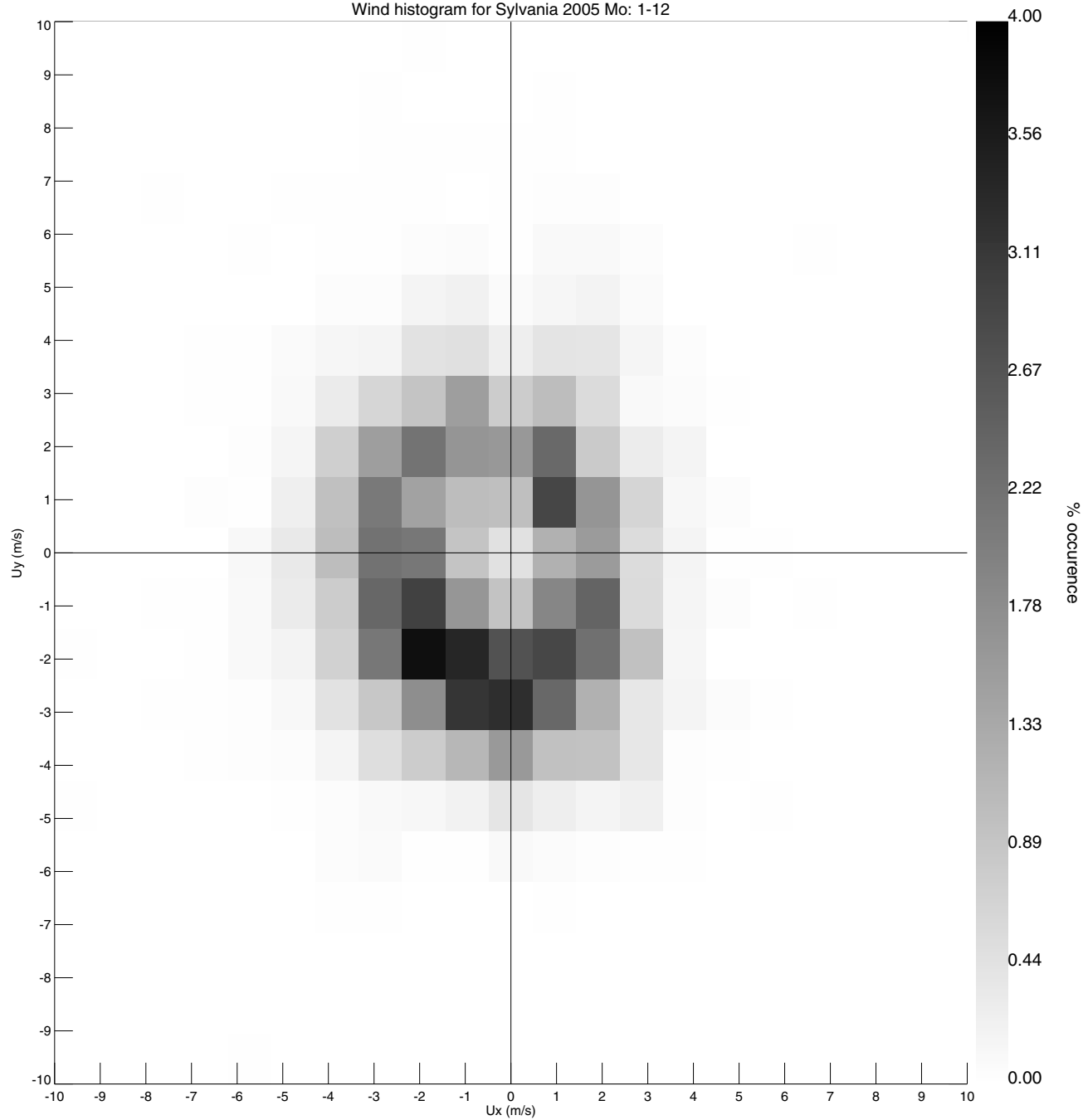
Wind histogram for Sylvania 2005 Mo: 1-12
