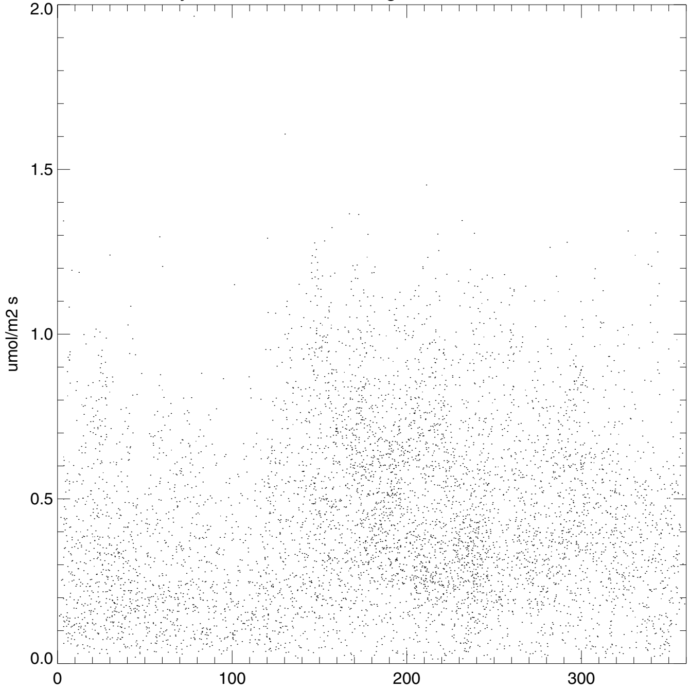
Sylvania Wind Dir vs. Night u^* 2005 Mo: 1-12
