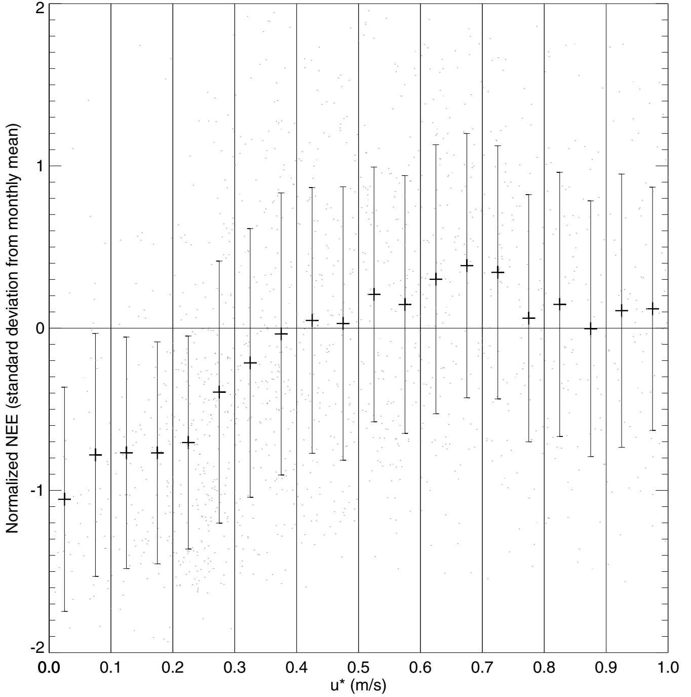
U* vs nighttime NEE Sylvania 2005 Month: 1-12 SOUTH
