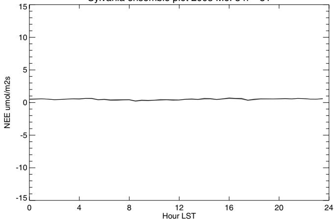
Sylvania ensemble plot 2005 Mo: 5 n = 31
