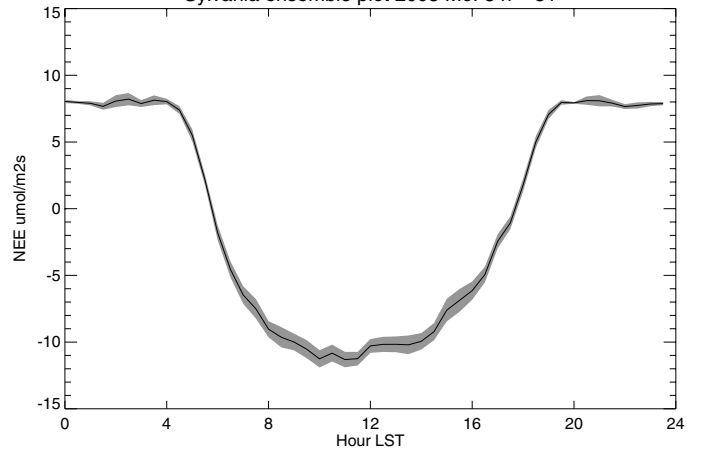
Sylvania ensemble plot 2005 Mo: 10 n = 31
