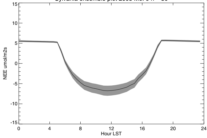
Sylvania ensemble plot 2005 Mo: 11 n = 30
