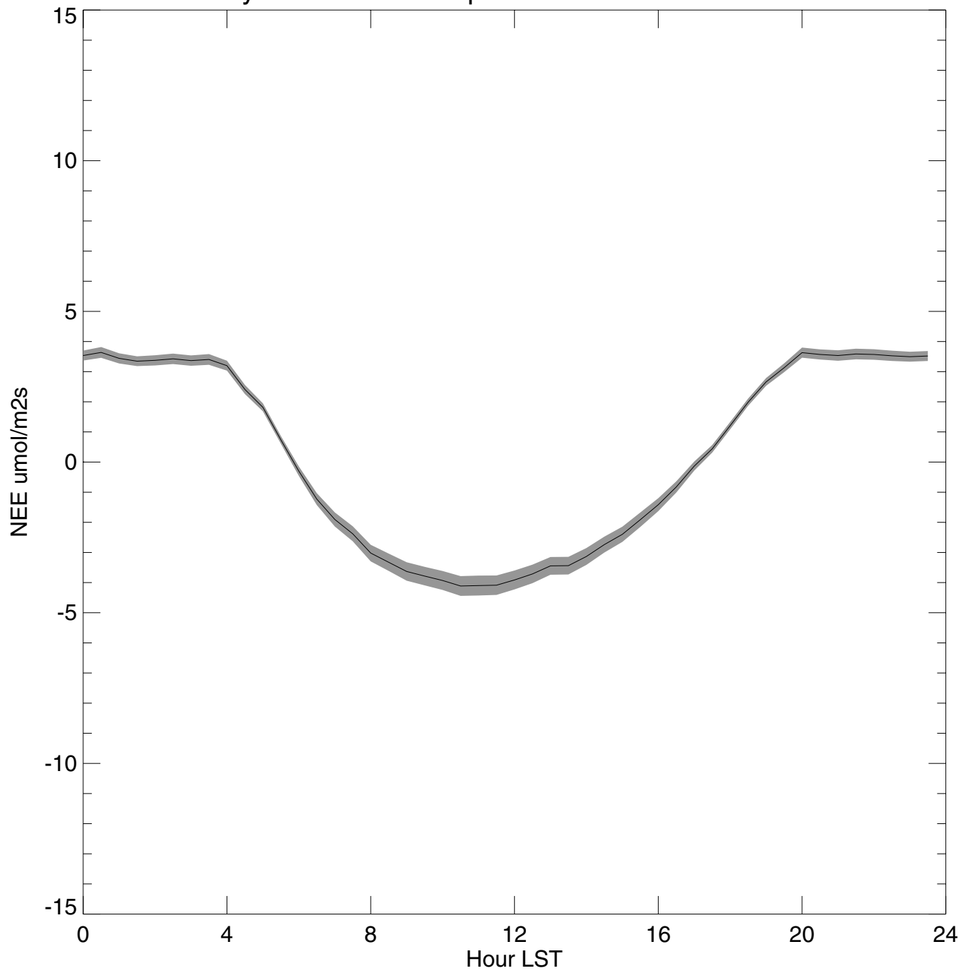
Sylvania ensemble plot 2005 Mo: 1-12 n = 365
