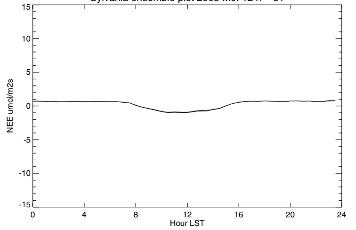
Sylvania ensemble plot 2005 Mo: 12 n = 31
