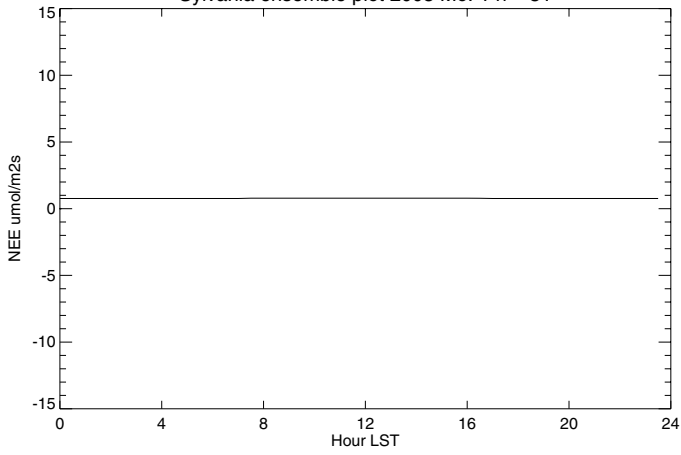
Sylvania ensemble plot 2005 Mo: 3 n = 31
