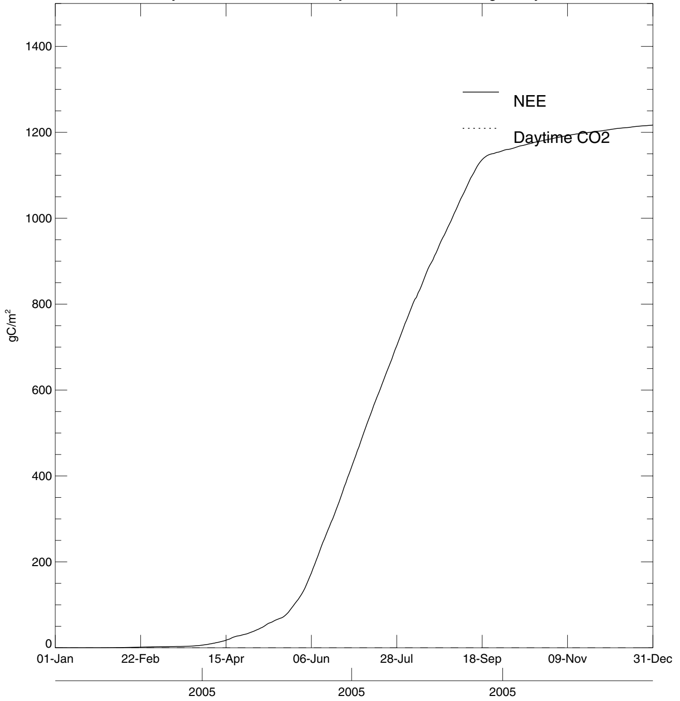
Sylvania cumulative GEPsyn 2005 Total: 1216.9 gC/m 2 yr
