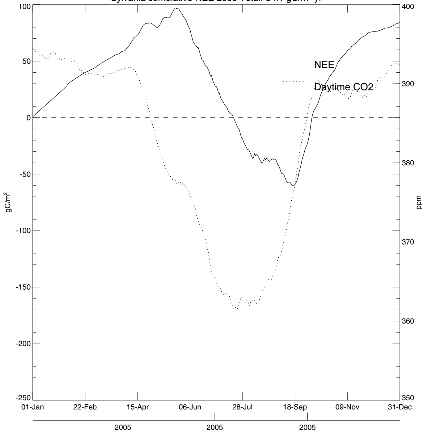
Sylvania cumulative NEE 2005 Total: 84.1 gC/m 2 yr
