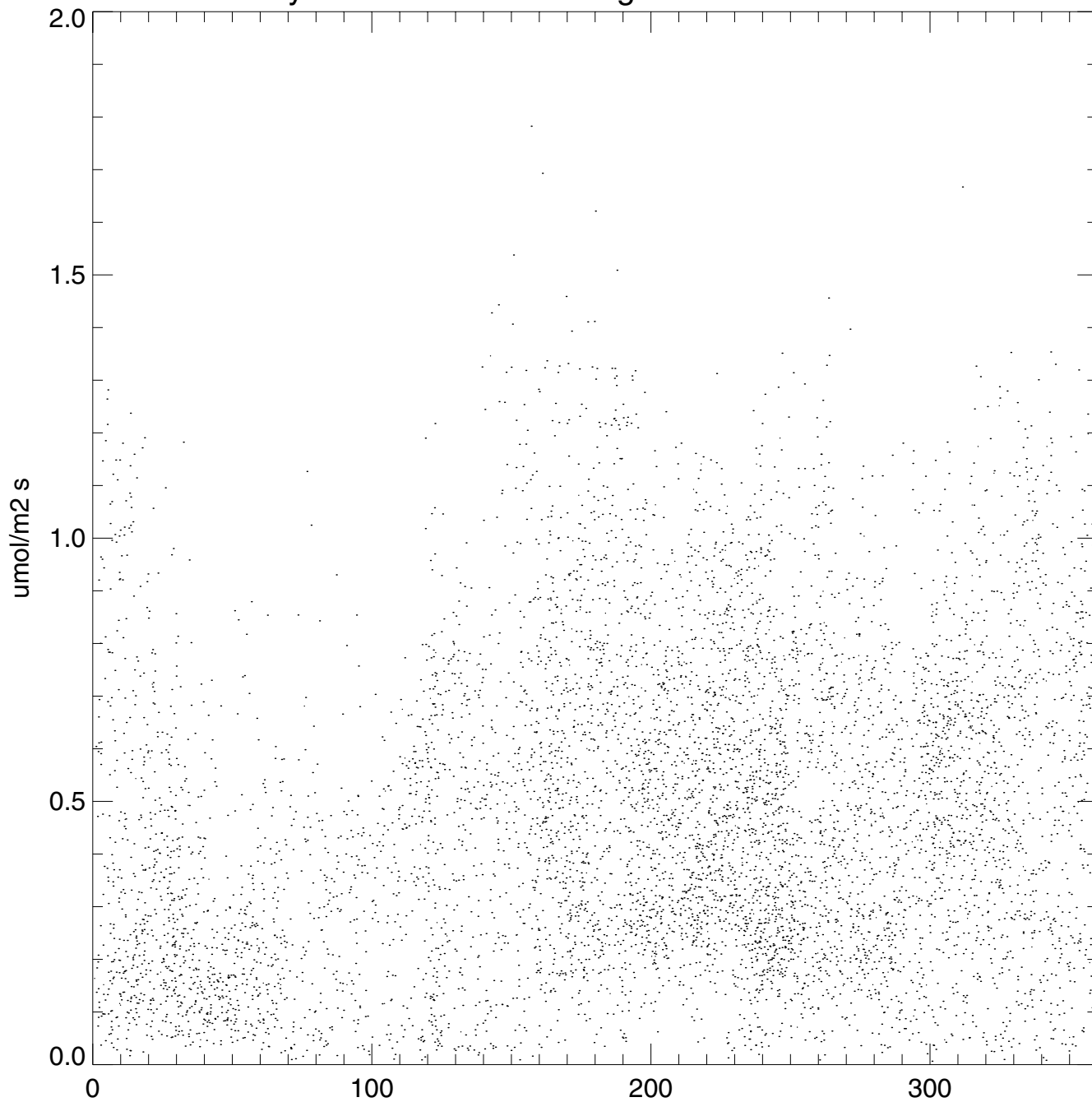
Sylvania Wind Dir vs. Night u^* 2004 Mo: 1-12
