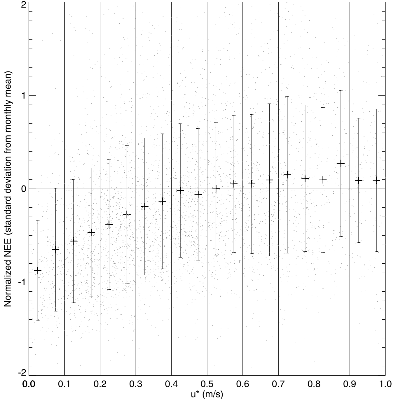
U* vs nighttime NEE Sylvania 2004 Month: 1-12
