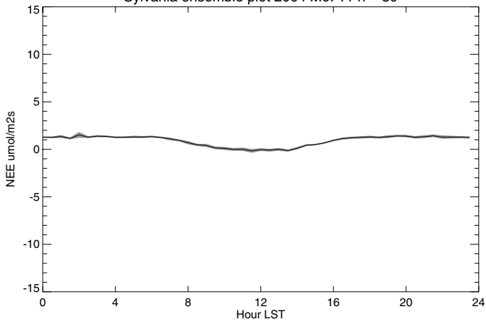
Sylvania ensemble plot 2004 Mo: 11 n = 30
