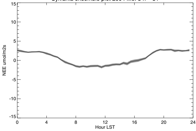
Sylvania ensemble plot 2004 Mo: 5 n = 31
