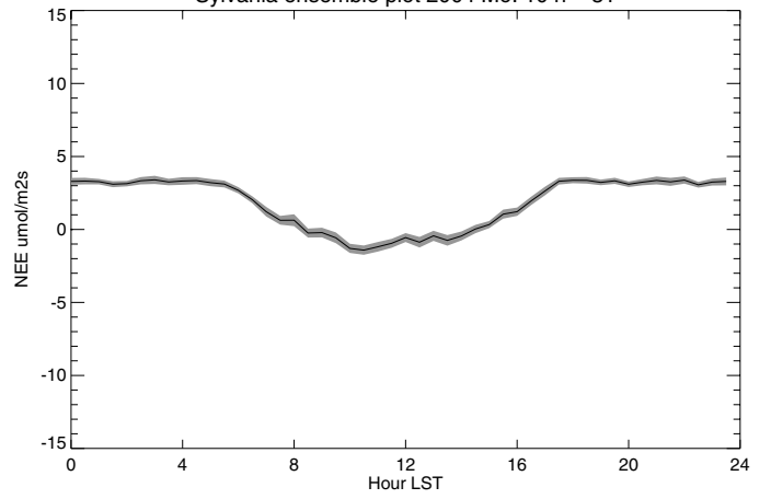
Sylvania ensemble plot 2004 Mo: 12 n = 31
