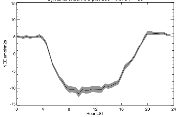
Sylvania ensemble plot 2004 Mo: 6 n = 30
