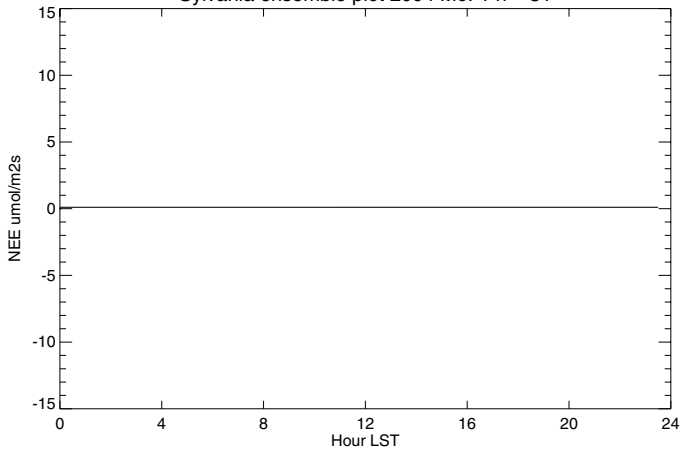
Sylvania ensemble plot 2004 Mo: 3 n = 31
