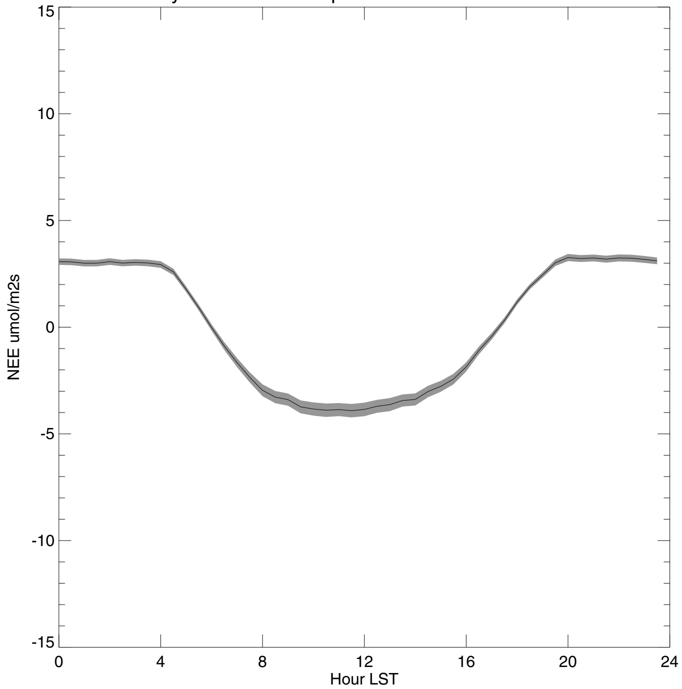
Sylvania ensemble plot 2004 Mo: 1-12 n = 366
