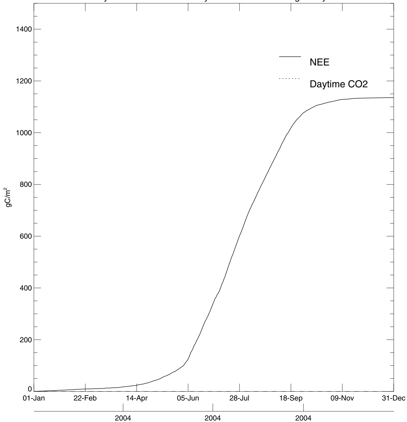
Sylvania cumulative GEPsyn 2004 Total: 1135.5 gC/m 2 yr
