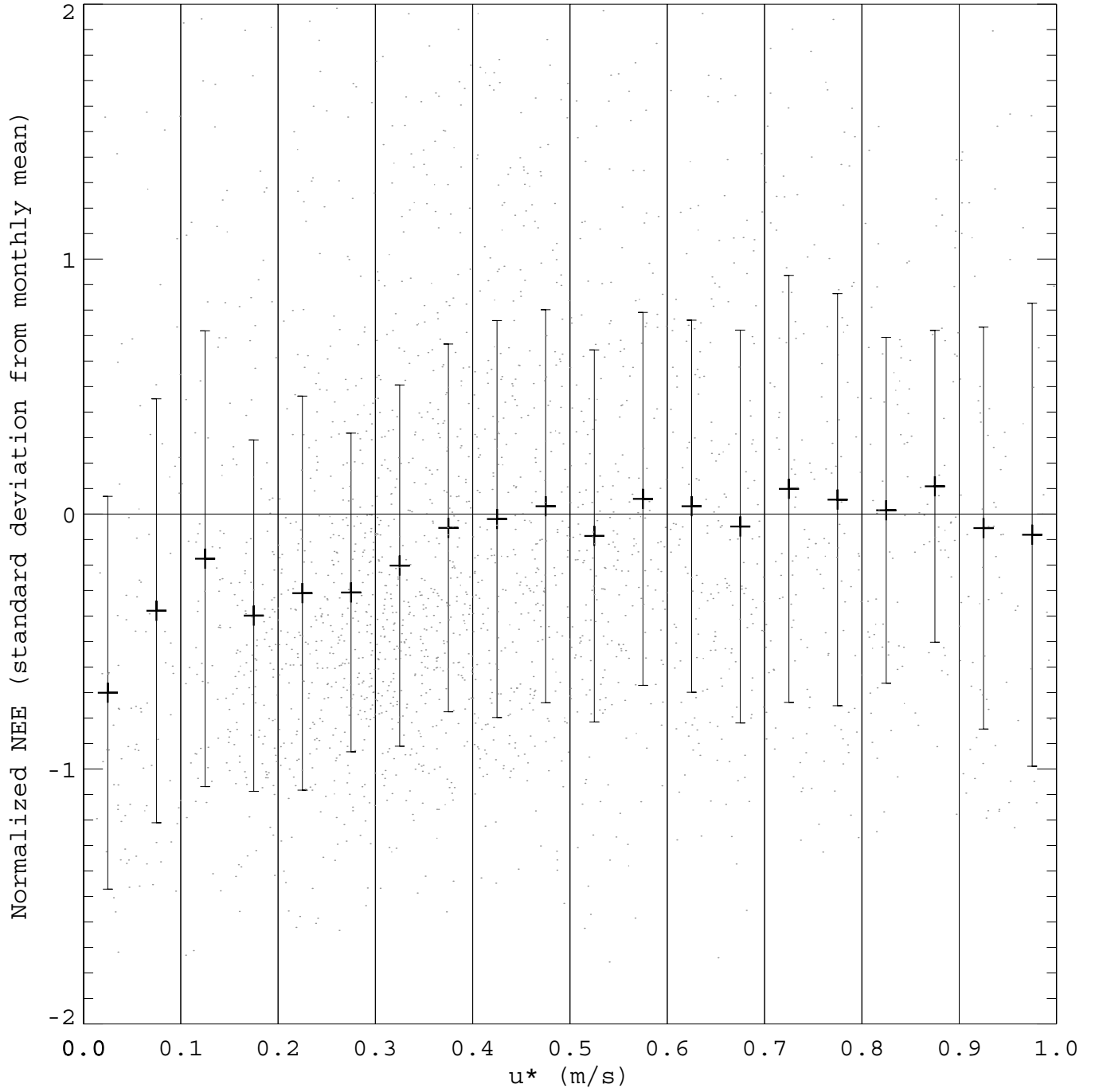
U* vs nighttime NEE Sylvania 2003 Month: 1-12 SOUTH
