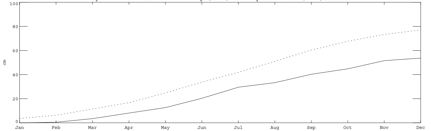
Sylvania 2003 Cumulative Precip (53.7) vs Marquette 61-90 (77.1)-dotted
