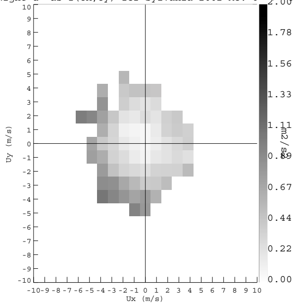
Night u^* as f(U_x, U_y) for Sylvania 2002 Mo: 6
