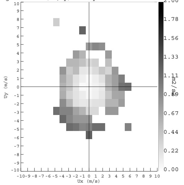
Night u^* as f(U_x, U_y) for Sylvania 2002 Mo: 3
