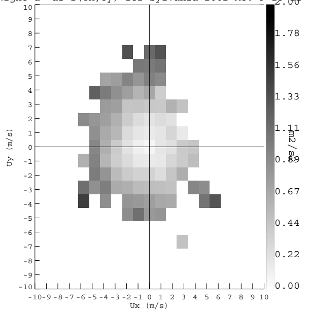
Night u^* as f(U_x, U_y) for Sylvania 2002 Mo: 9
