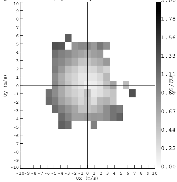
Night u^* as f(U_x, U_y) for Sylvania 2002 Mo: 12
