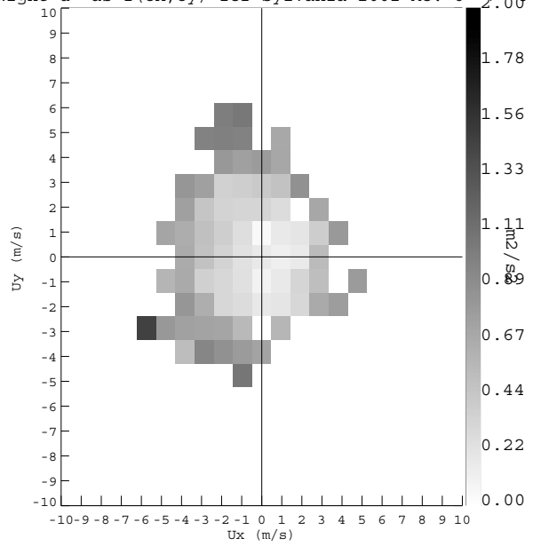
Night u^* as f(U_x, U_y) for Sylvania 2001 Mo: 6 27.00 8
