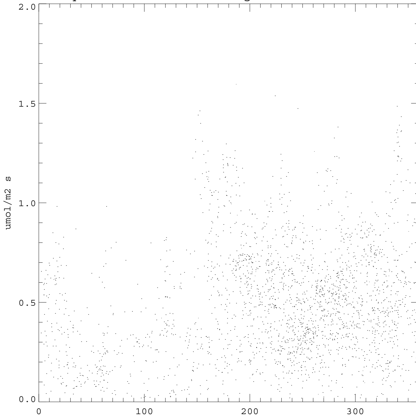
Sylvania Wind Dir vs. Night u^* 2001 Mo: 1-12
