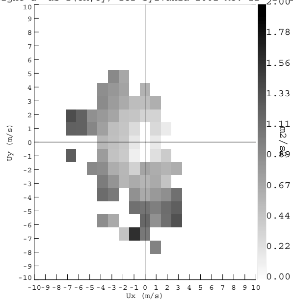
Night u^* as f(U_x, U_y) for Sylvania 2001 Mo: 12 21.00 2
