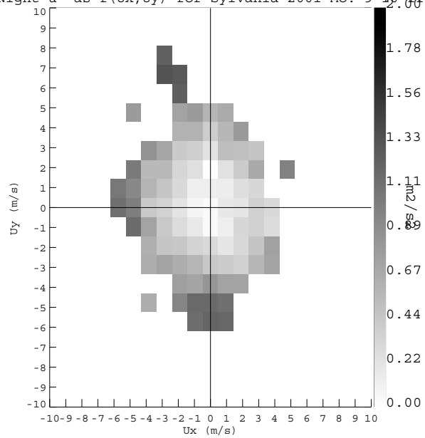
Night u^* as f(U_x, U_y) for Sylvania 2001 Mo: 9 10.00 11
