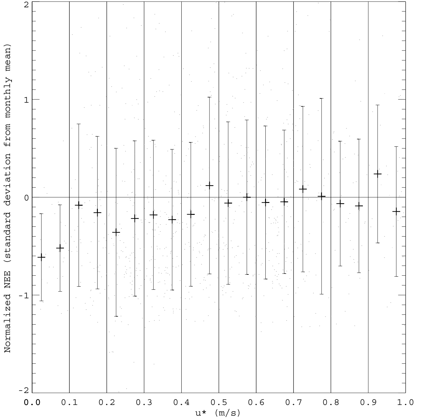
U* vs nighttime NEE Sylvania 2001 Month: 1-12
