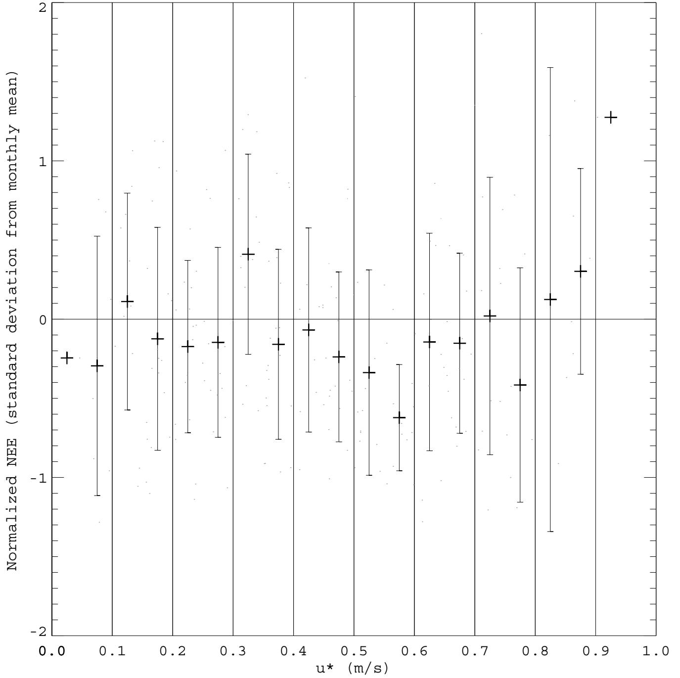
U* vs nighttime NEE Sylvania 2001 Month: 1-12 NORTH
